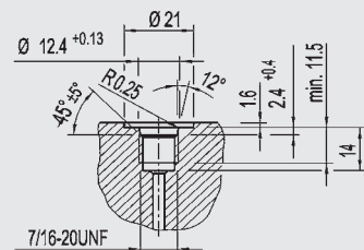
7/16-20 UNF
