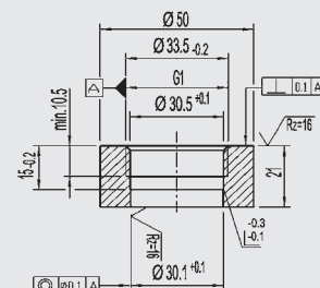
G 1, with O-ring 1) 2)
