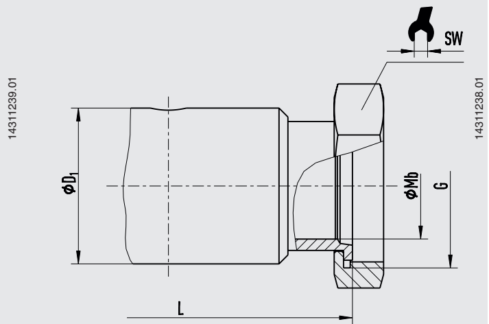
Union nut
