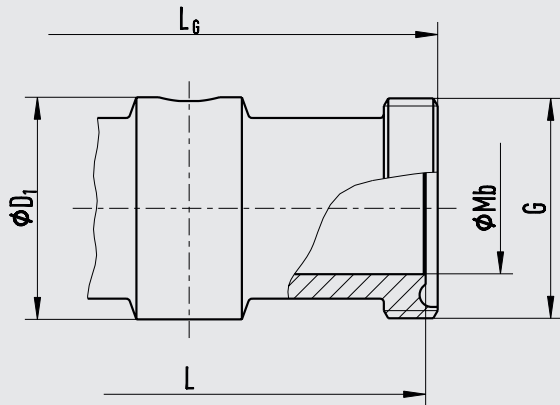
Threaded coupling
