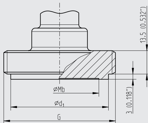
Threaded coupling
