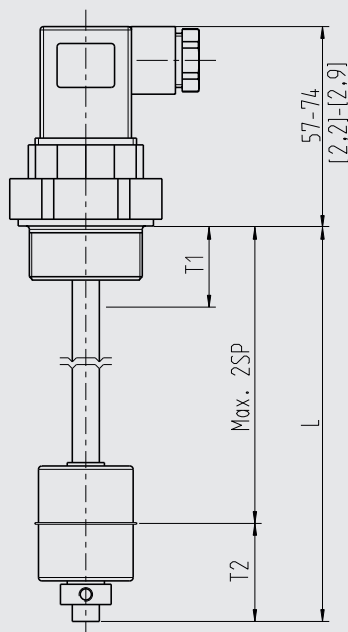
with angular connector form A
